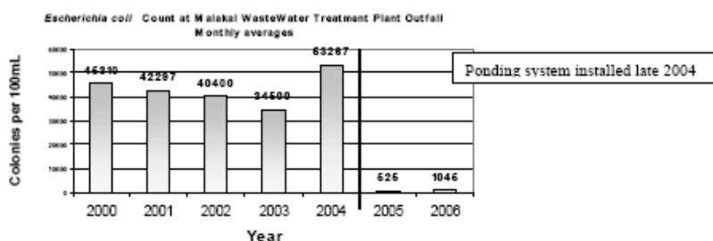
Figure 3: Faecal Coliform indicator counts, Malakal WWTP outfall, Malakal Channel. (Source: Palau EQPB)
